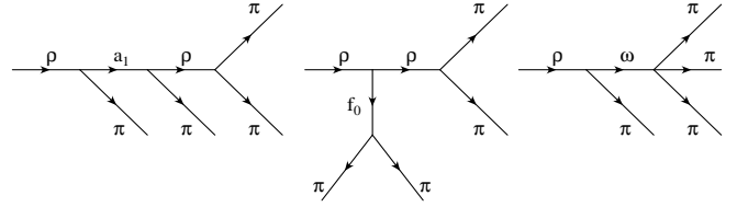
Fig. 4. Diagrams contributing to the hadronic current
