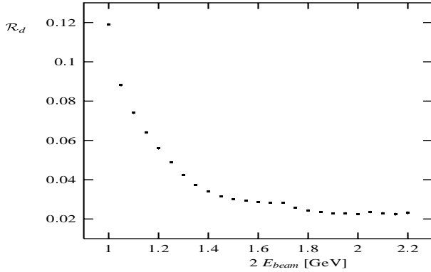
Fig. 3. The ratio \mathcal{R}_d \equiv (\sigma_1 - \sigma_2)/\sigma_2 , where \sigma_1 ( \sigma_2 ) is the e^+e^- \rightarrow 2\pi^0\pi^-\pi^+ cross section calculated for true pion masses (with all masses equal to m_- )
