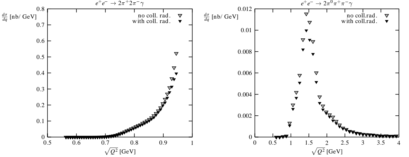
Fig. 9. The effect of the collinear radiation on the differential e^+e^- \rightarrow 4\pi\gamma cross sections at beam energy 0.5 GeV (left picture) and 5 GeV (right picture) with minimal photon energy equal to 0.05 and 0.2 GeV, respectively. In the mode with collinear radiation minimal invariant masses of the 4\pi + \gamma systems of 0.95 GeV and 9.5 GeV were required. q \equiv \sqrt{Q^2} denotes the invariant mass of the 4\pi system
