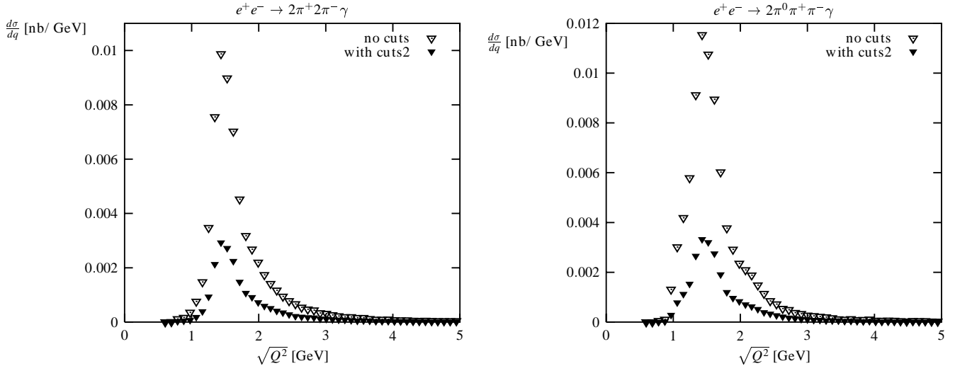
Fig. 8. The differential e^+e^- \rightarrow 4\pi\gamma cross sections at beam energy 5 GeV with minimal photon energy equal 0.2 GeV with no cuts on pions angles and 7^\circ < \theta_\gamma < 173^\circ (no cuts) and angular cuts of (40) (with cuts2), where q \equiv \sqrt{Q^2} is an invariant mass of the 4\pi system
