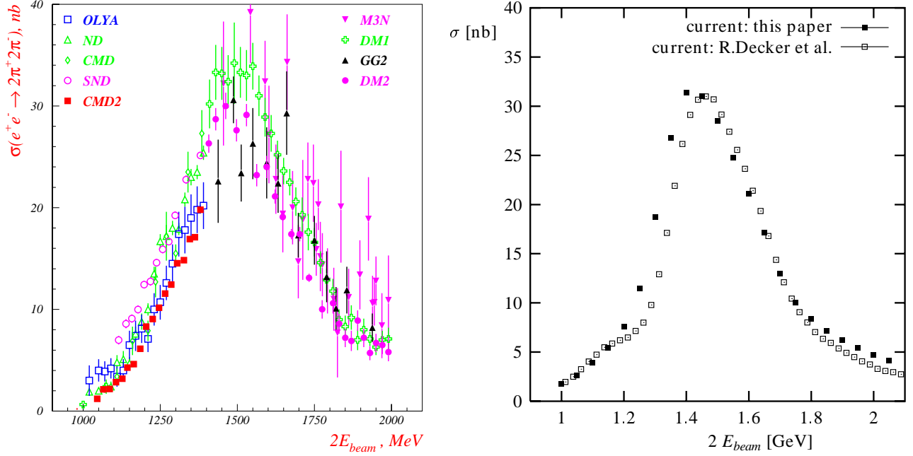
Fig. 5. Comparison of data (left figure, see text) and predictions (right figure) obtained using the current (32) (filled squares) and those of [11] (empty squares), respectively, for \sigma(e^+e^- \rightarrow 2\pi^+2\pi^-)
