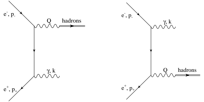
Fig. 1. Diagrams contributing to the process e^+e^- \rightarrow \gamma + \text{hadrons} (only initial state radiation included)
