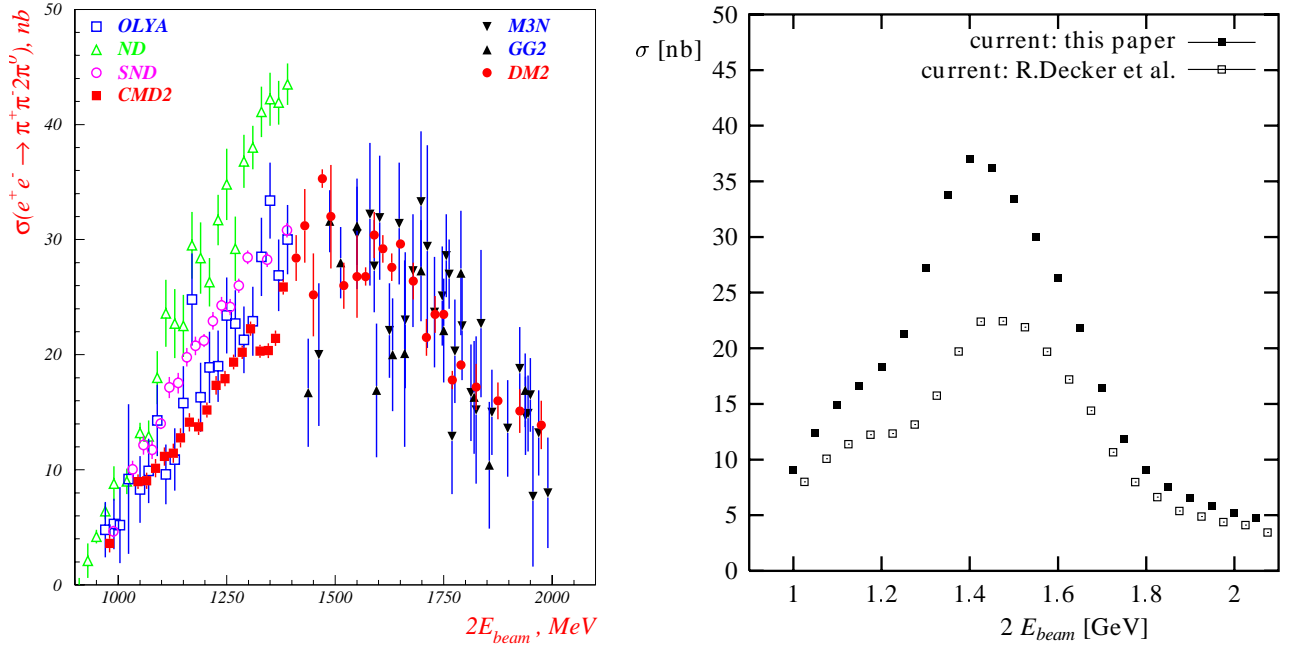
Fig. 6. Comparison of data (left figure, see text) and predictions (right figure) obtained using the current (32) (filled squares) and those of [11] (empty squares), respectively, for \sigma(e^+e^- \rightarrow \pi^+\pi^-2\pi^0)
