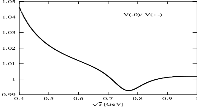
Fig. 2. The ratio of the two spectral functions (see text for explanation)
