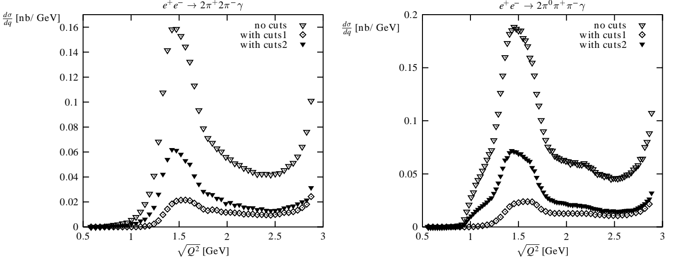
Fig. 7. The differential e^+e^- \rightarrow 4\pi\gamma cross sections at beam energy 1.5 GeV with minimal photon energy equal 0.1 GeV with no cuts on pions angles and 7^\circ < \theta_\gamma < 173^\circ (no cuts) and two sets of angular cuts (39) (with cuts1) and (40) (with cuts2), where q \equiv \sqrt{Q^2} is an invariant mass of the 4\pi system
